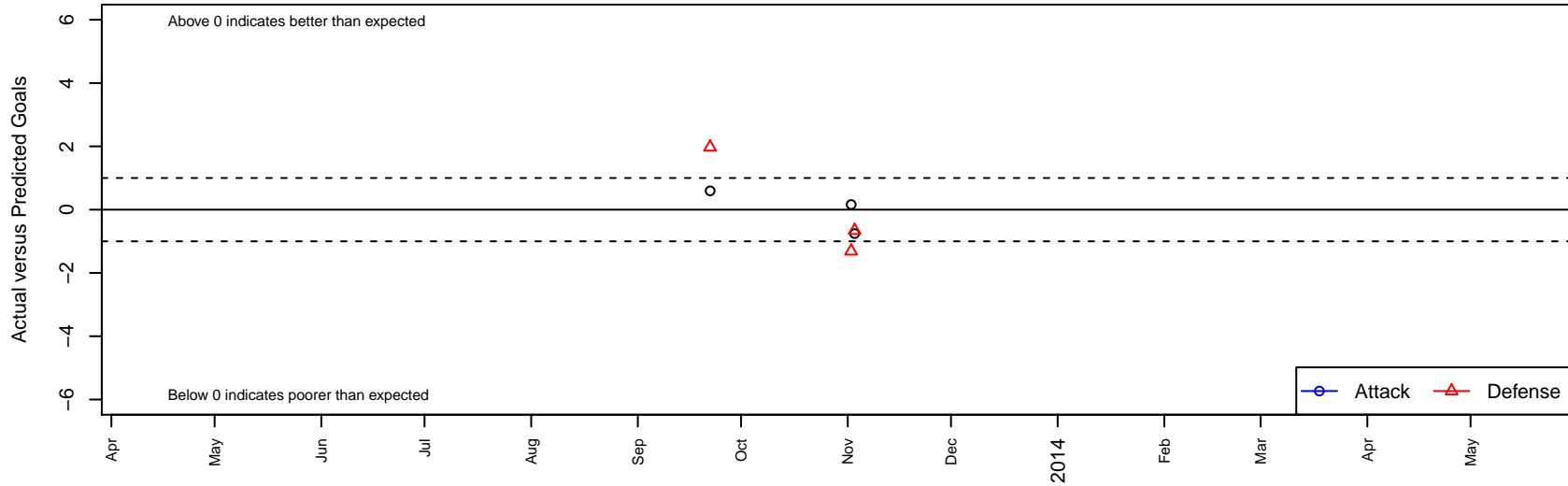
Union City SC Juventus B98 Dots are actual minus expected GF (blue circles) and GA (red triangles). Blue line is smoothed change in attack strength. Red is smoothed change in defense strength.
